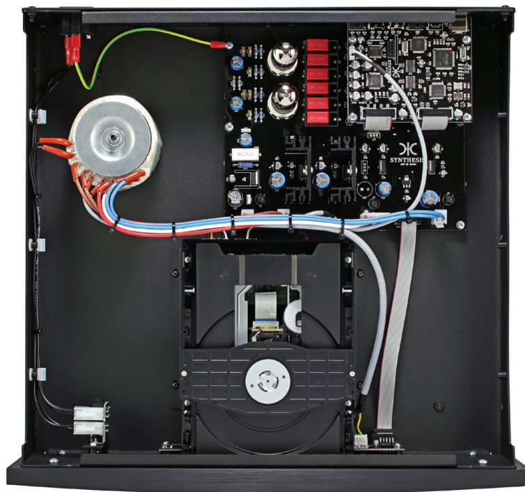
At left a toroidal mains transformer to provide power and at top-centre two ECC88 low noise double-triode output valves that deliver a lower than common 1.5V output. At bottom centre, a high quality Teac CD transport mechanism.
